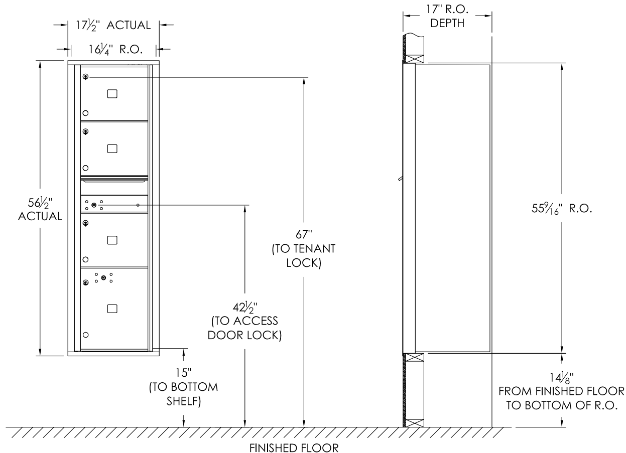
COMPARTMENT CHART
