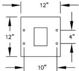
PEDESTAL BASE BOLT PATTERN
