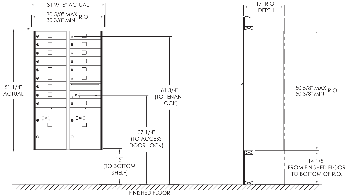
COMPARTMENT CHART
