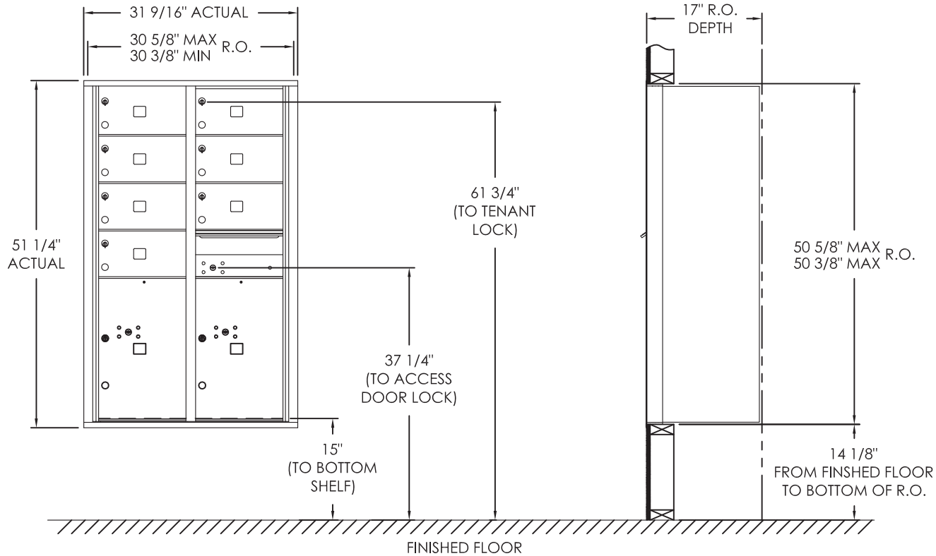
COMPARTMENT CHART
