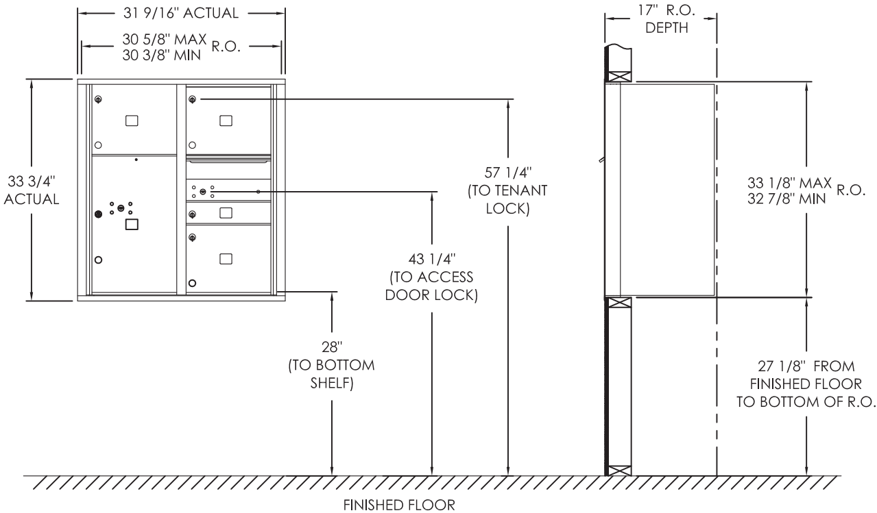
COMPARTMENT CHART
